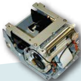
Steel frame, metal components, and self-sharpening ceramic knife
